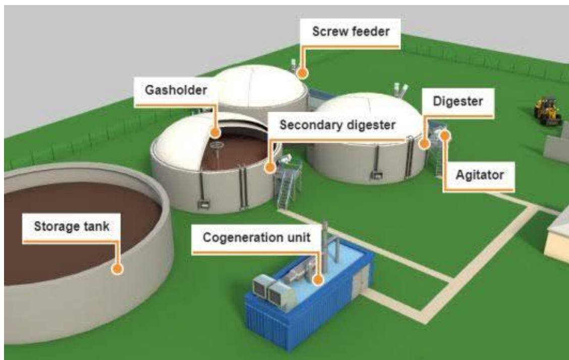
Fig 3: Biomass Energy Plant
