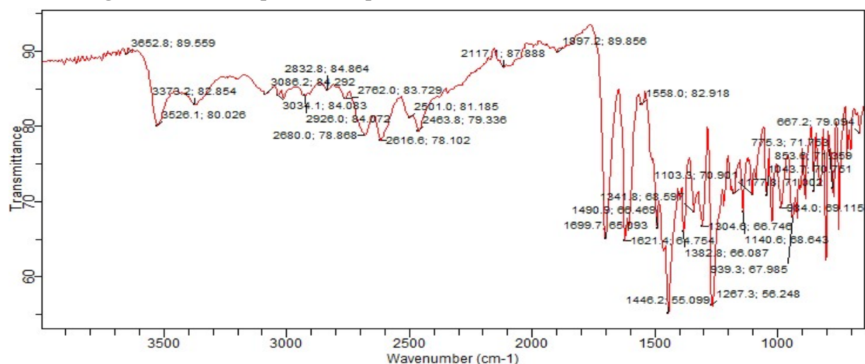
Figure 3.2: FT-IR Spectra of Ciprofloxacin
