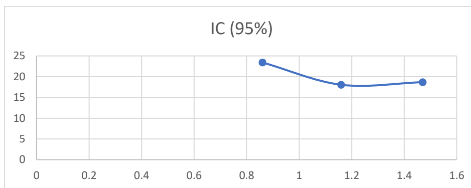
Fig 3.14: shows the graph of Log concentrations of ciprofloxacin+ Irvingia gabonensis against IC95% mean inhibition of K. pneumoniae
